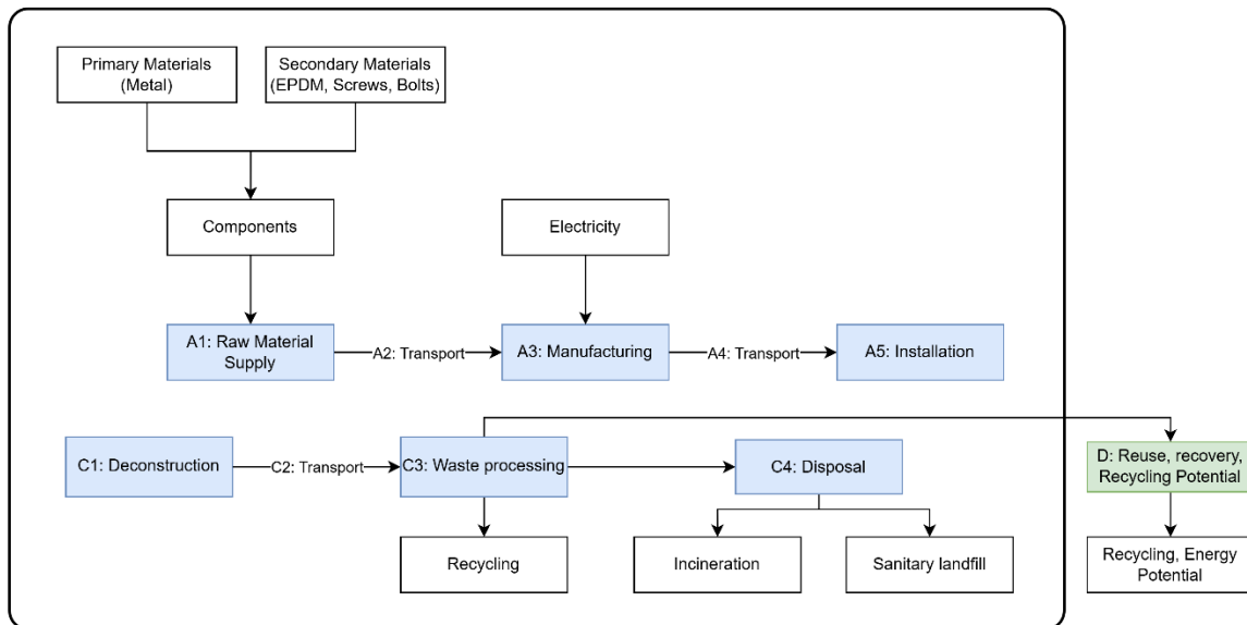
Figure 4 - Overall lifecycle flow.
