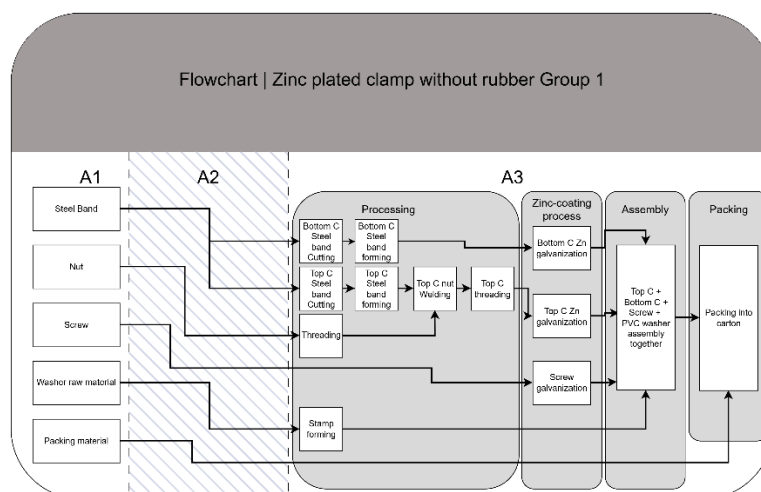
Figure 5 - Manufacturing-specific process flow.
